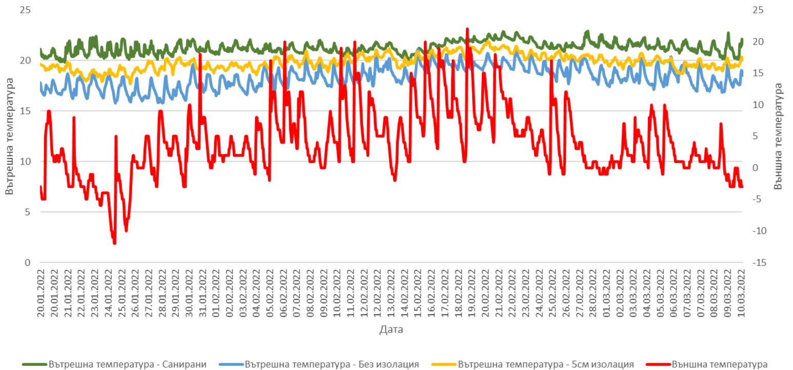
Comparison internal / external temperature
